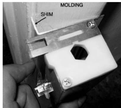
Molding shim for clamshell door molding. Long screws mount directly through shim.
