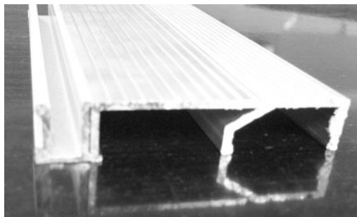
Flat Threshold- Shown between lower guide rail and the standard threshold (normally the customers existing threshold)
