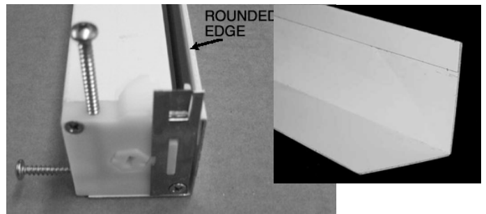
Housing back cover plate. Used when the fourth side of the housing is exposed to elements (blowing sand, volcanic ash, etc)
